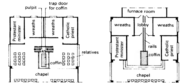
⑥ Layout with furnace room beneath the chapel
